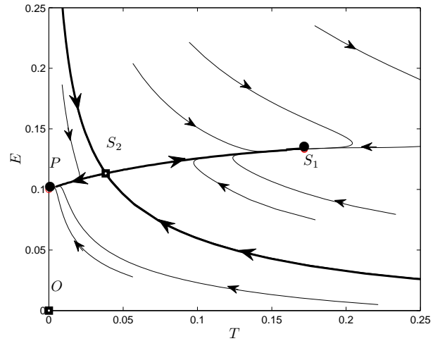
Figure 5: The dynamics in the phase space of (1), with K = .1 , \alpha = 0.01 , r = .01 , a = .03 , \sigma = 0.2 , \beta = 0.0215 , \rho = 0.2
