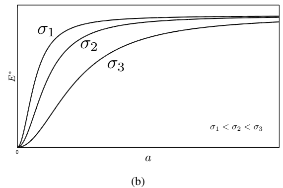
Figure 3: Comparative static on the parameter \sigma
