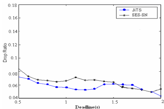
Fig.3 Drop Ratio of SES-SN and JiTS
