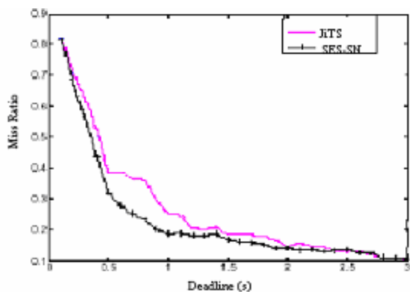
Fig. 9 Miss Ratio of SES-SN and JiTS under bursty traffic
