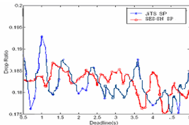
Fig. 6 Drop Ratio of SES-SN and JiTS with SP
